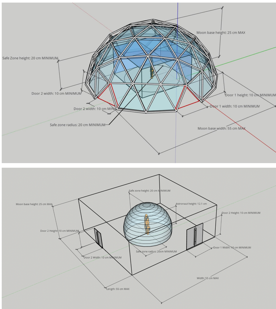
Fig 1. Clearances and dimensional specifications for space to fit the structure. These diagrams are a representation to show the MINIMUM interior dimensions of structures for the safe zone and MAXIMUM exterior dimensions of the Moon Base. Please note that the interior and exterior shape and placement of the openings/doors of the Moon Base is to be determined by teams within the minimum and maximum requirements.
