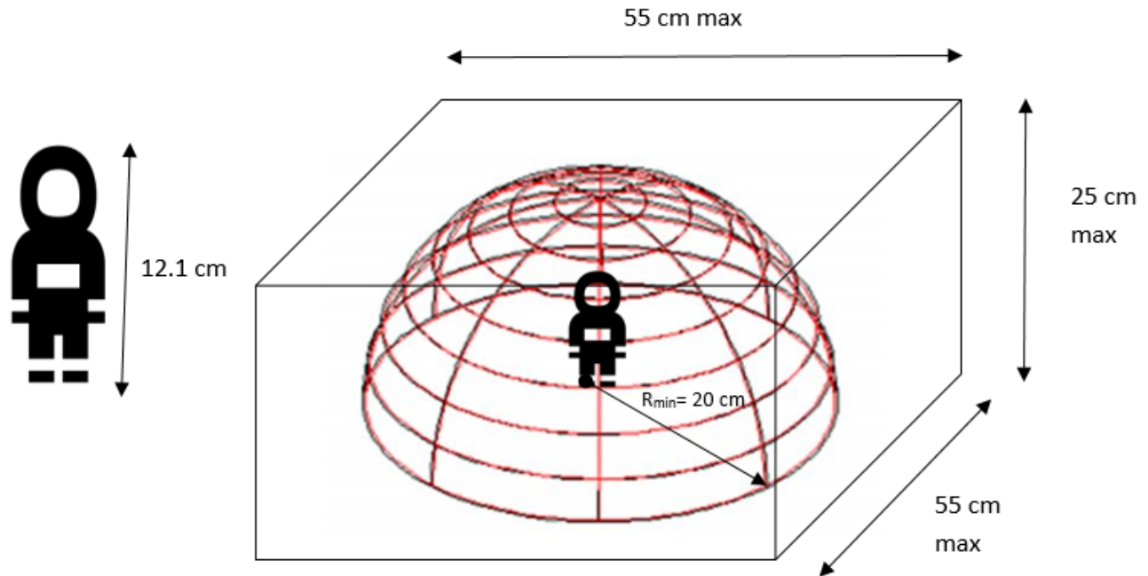
Fig 1. Clearances and dimensional specifications for space to fit the structure.
